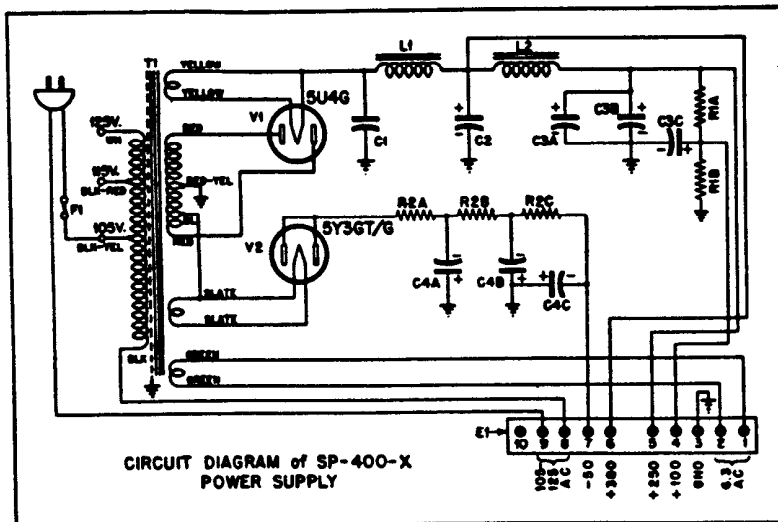
FIG. 10— Power supply diagram.
