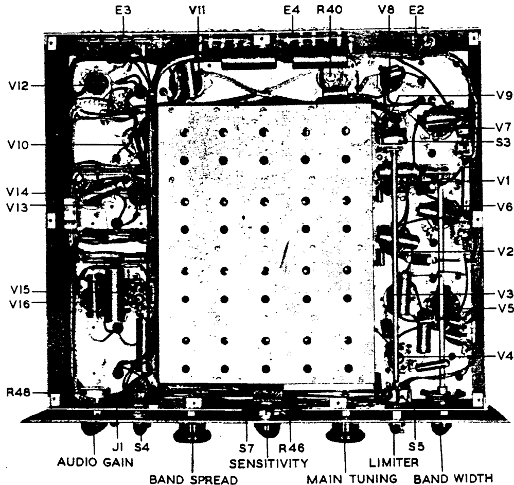
FIG. 12—Bottom view of chassis.
