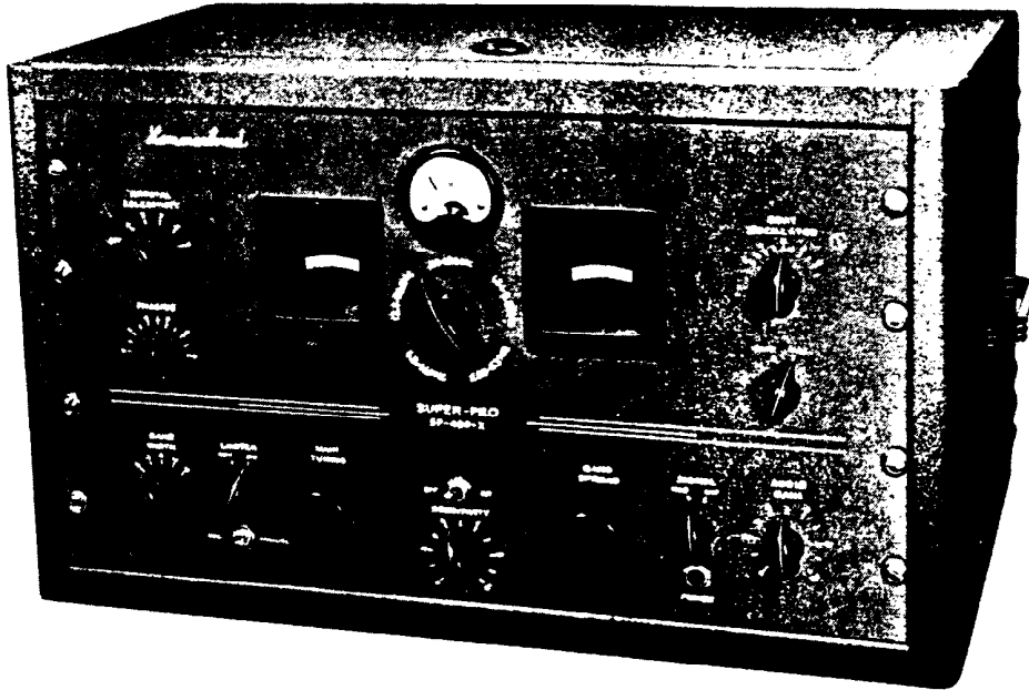
FIG. 1—Front view of "Super-Pro" model SP-400-X.
