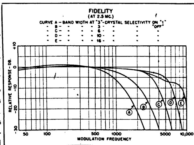
FIG. 9—Audio fidelity curves.
